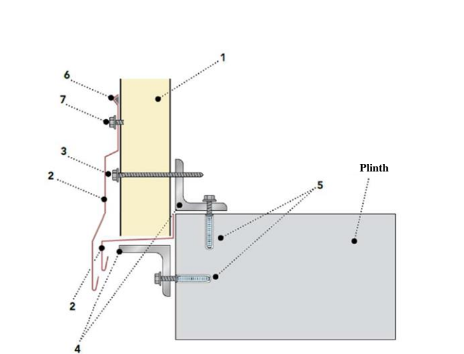
1b - Installation of wall panels on the outside of the plinth in a vertical position
