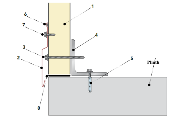
1a - Installation of wall panels on the plinth in a vertical position
